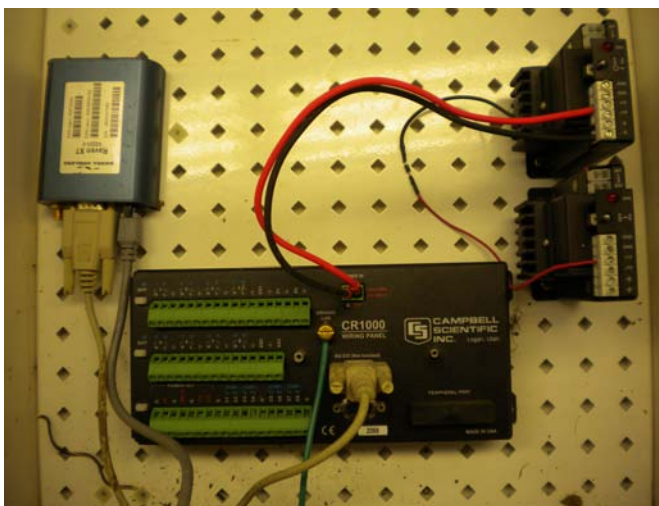
Figure 2.5. Photo of the “white box” contents. The object in the upper left is the cellular modem, the object in the middle is the data logger, and the two objects in the upper right are charge controllers.
